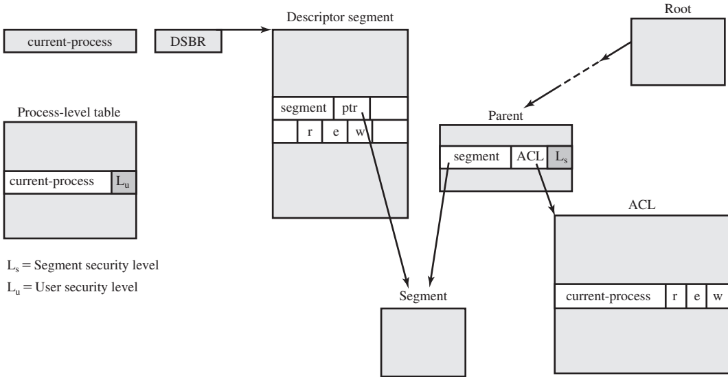
Figure 27.3 Multics Data Structures for MLS
