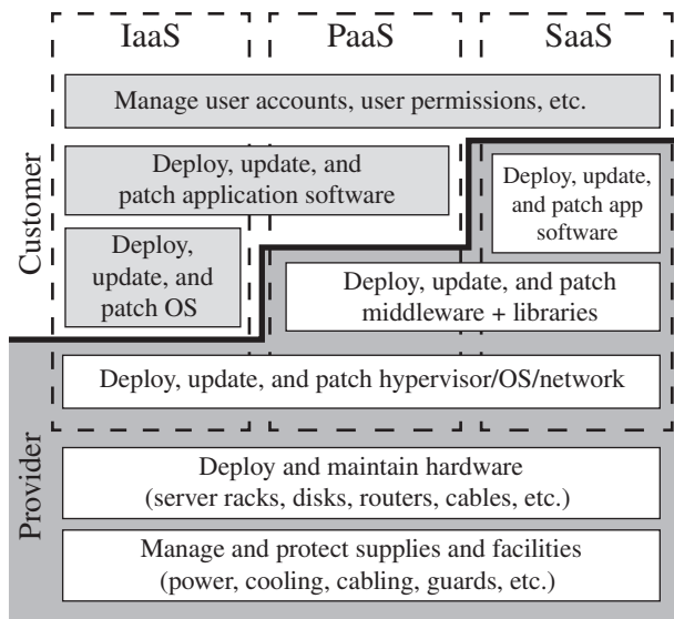
(b) Cloud computing management tasks
