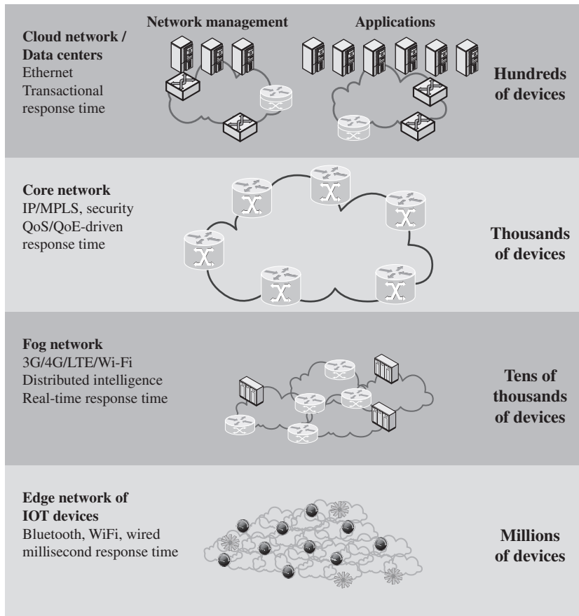
Figure 13.9 The IoT and Cloud Context
