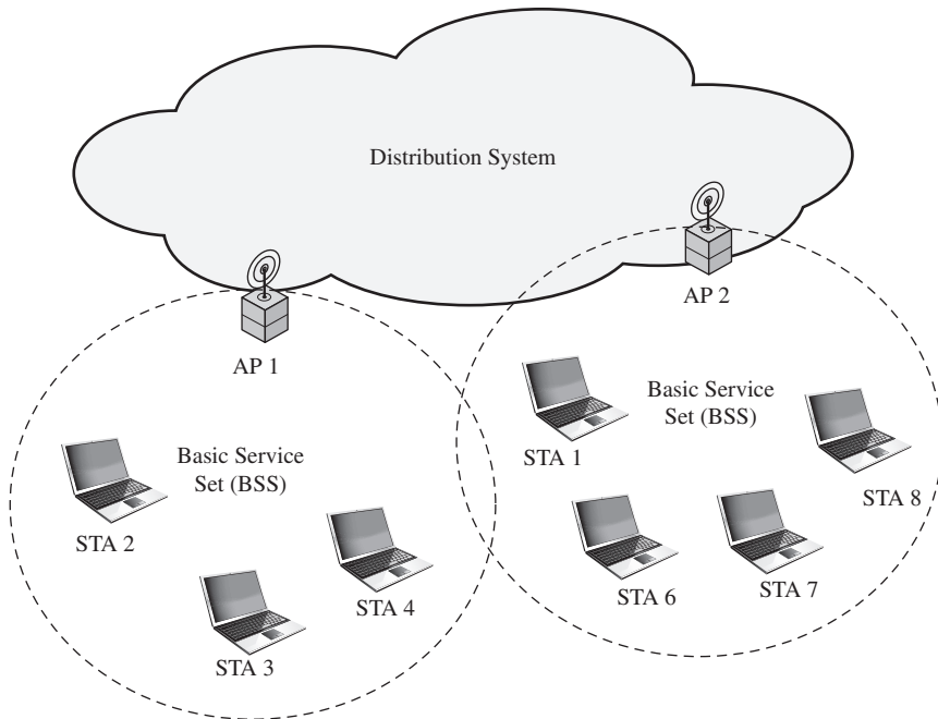
Figure 24.5 IEEE 802.11 Extended Service Set
