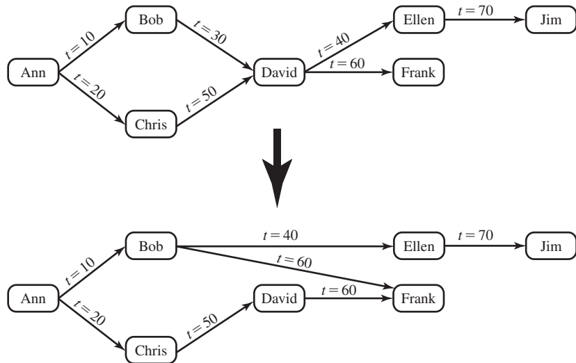
Figure 5.16 Bob Revokes Privilege from David, Second Version
