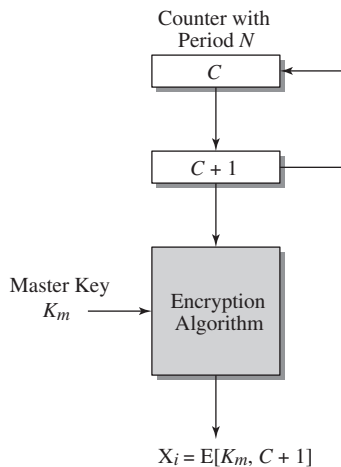
Figure D.1 Pseudorandom Number Generation from a Counter
