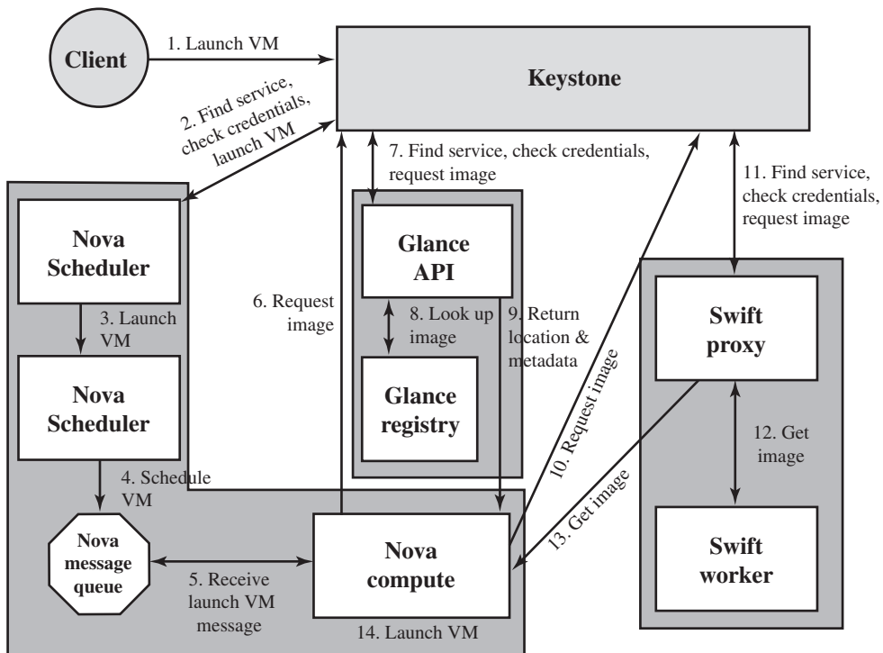
Figure 13.7 Launching a Virtual Machine in OpenStack
