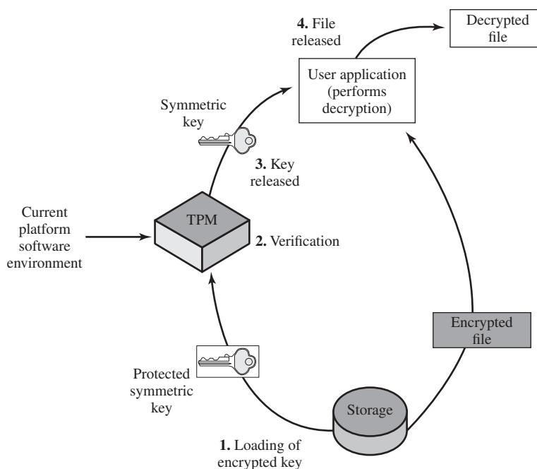
Figure 27.12 Decrypting a File Using a Protected Key
