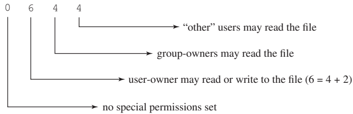
Figure 25.2 Permissions on mycoolfile
