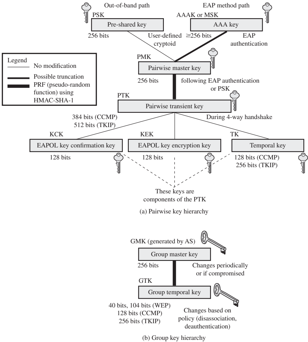
Figure 24.10 IEEE 802.11i Key Hierarchies
