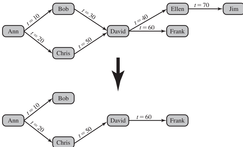
Figure 5.6 Bob Revokes Privilege from David
