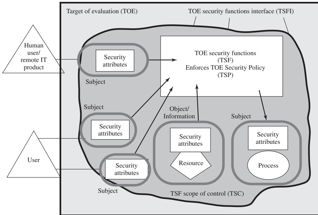
Figure 27.14 Security Functional Requirements Paradigm
