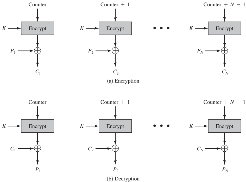
Figure 20.9 Counter (CTR) Mode
