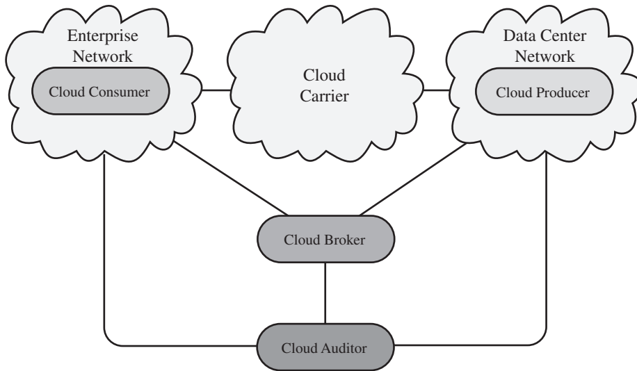
Figure 13.4 Interactions between Actors in Cloud Computing
