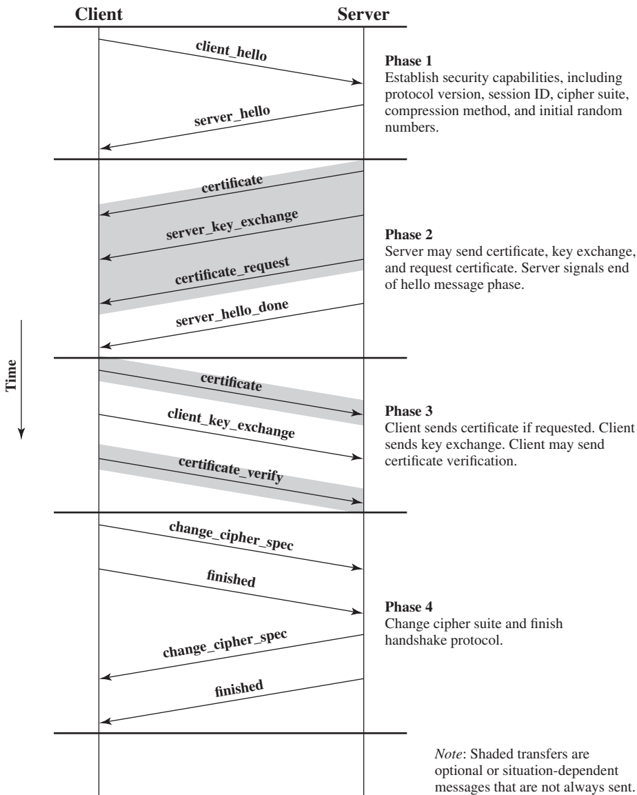
Figure 22.6 Handshake Protocol Action
