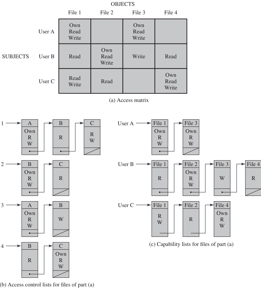
Figure 4.2 Example of Access Control Structures
