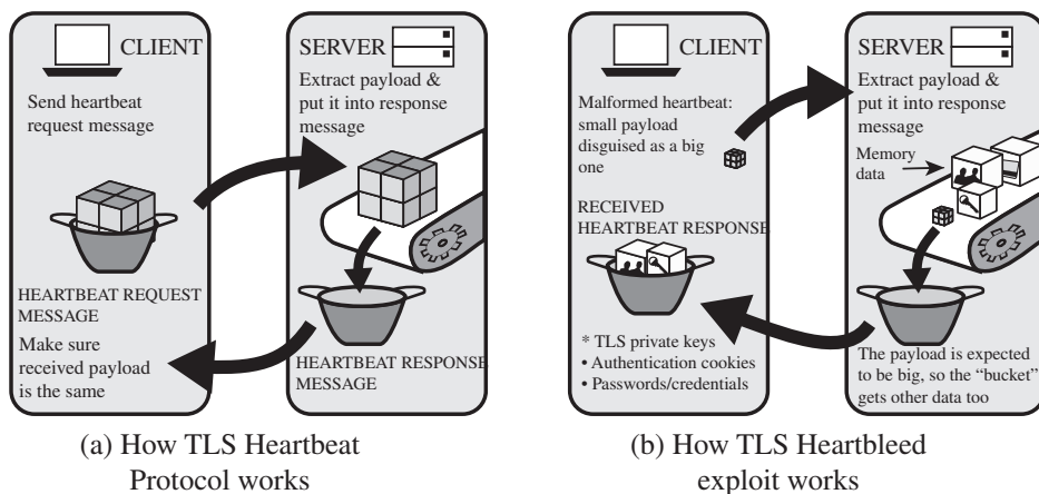
Figure 22.7 The Heartbleed Exploit
