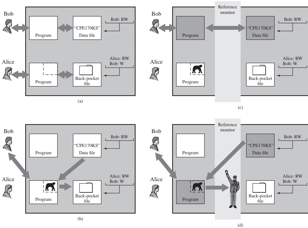
Figure 27.8 Trojan Horse and Secure Operating System
