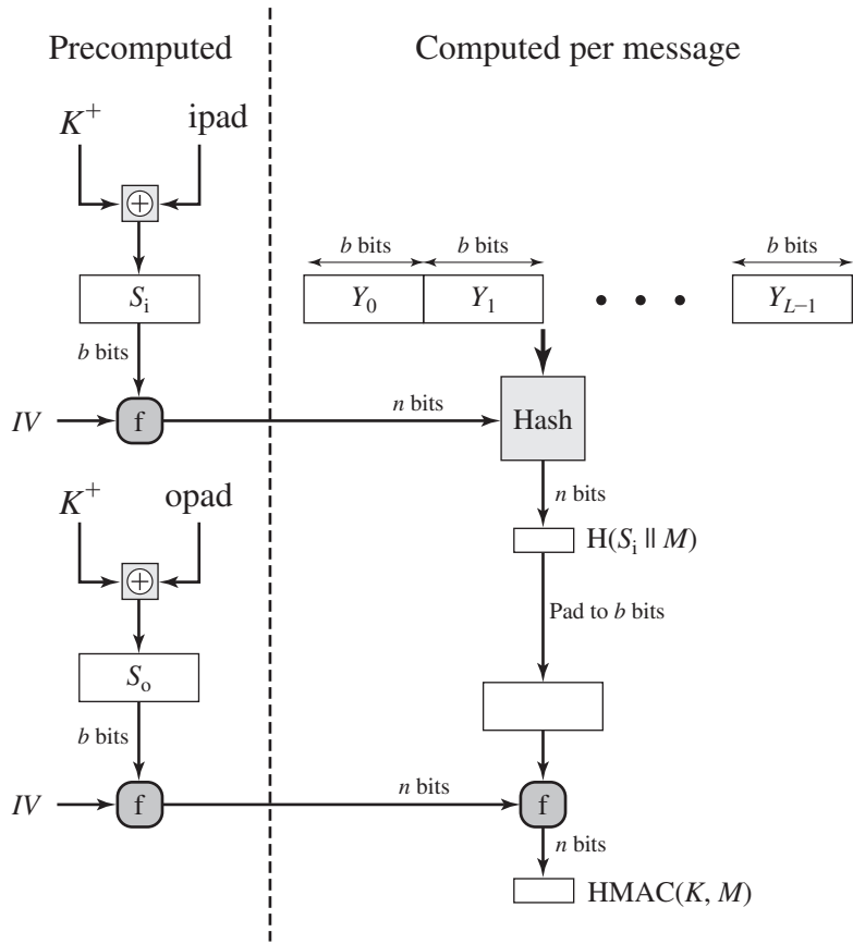
Figure 21.11 Alternative Implementation of HMAC
