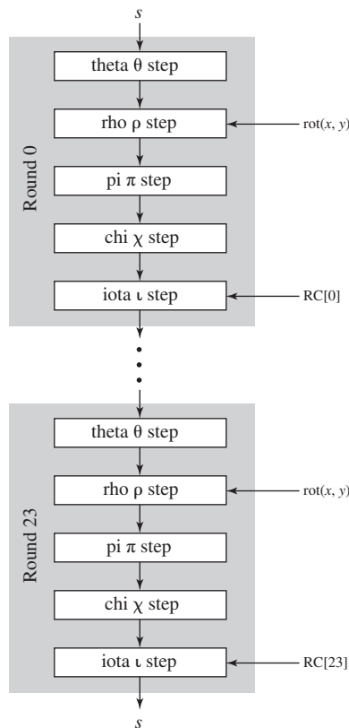
Figure J.4 SHA-3 Iteration Function f
