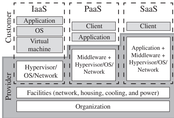
(a) Cloud computing assets
