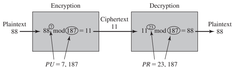
Figure 21.8 Example of RSA Algorithm
