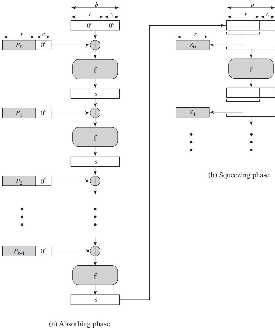
Figure J.2 Sponge Construction
