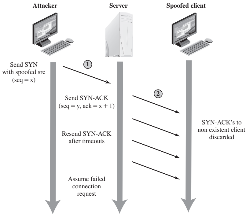
Figure 7.3 TCP SYN Spoofing Attack
