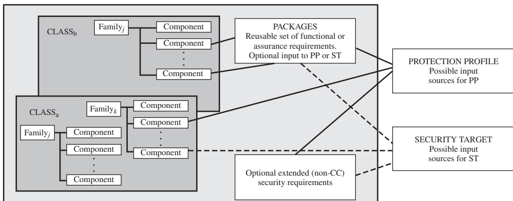
Figure 27.13 Organization and Construction of Common Criteria Requirements
