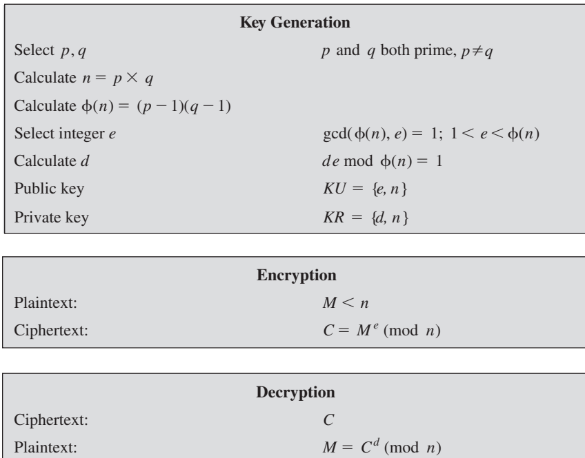
Figure 21.7 The RSA Algorithm
