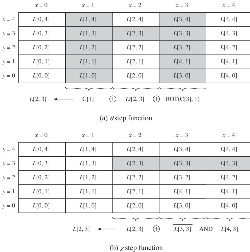
Figure J.5 Theta and Chi Step Functions
