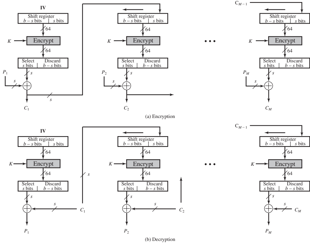
Figure 20.8 s -bit Cipher Feedback (CFB) Mode
