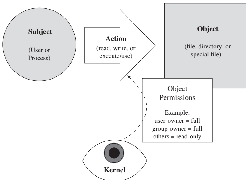
Figure 25.1 Linux Security Transactions
