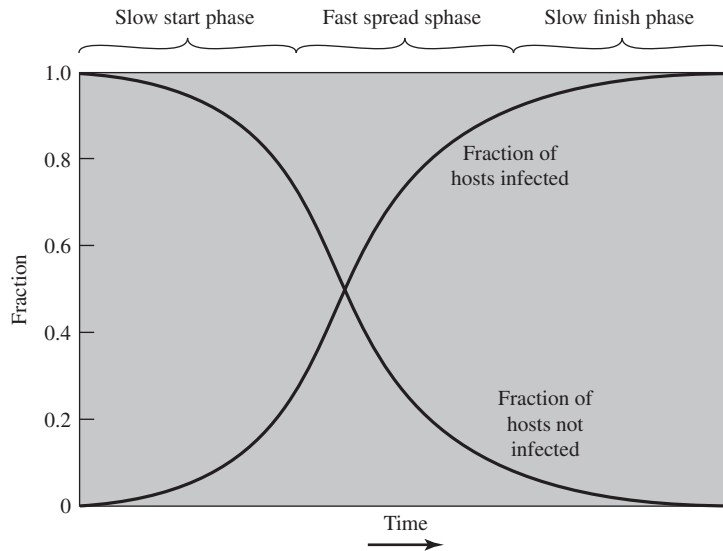
Figure 6.2 Worm Propagation Model
