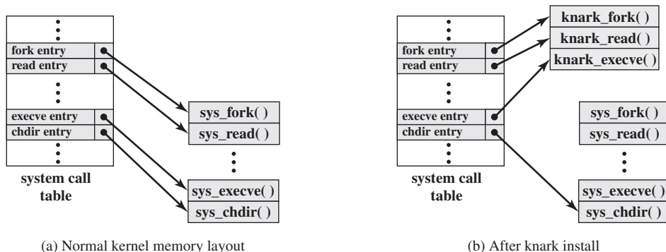
Figure 6.3 System Call Table Modification by Rootkit
