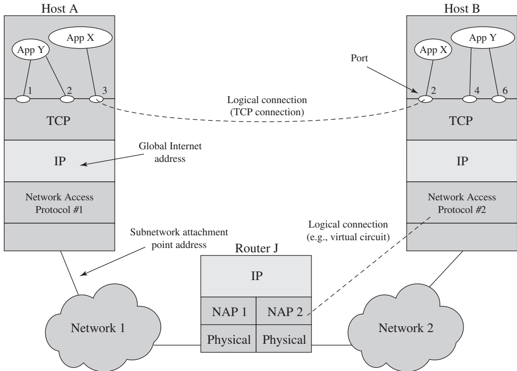
Figure F.2 TCP/IP Concepts
