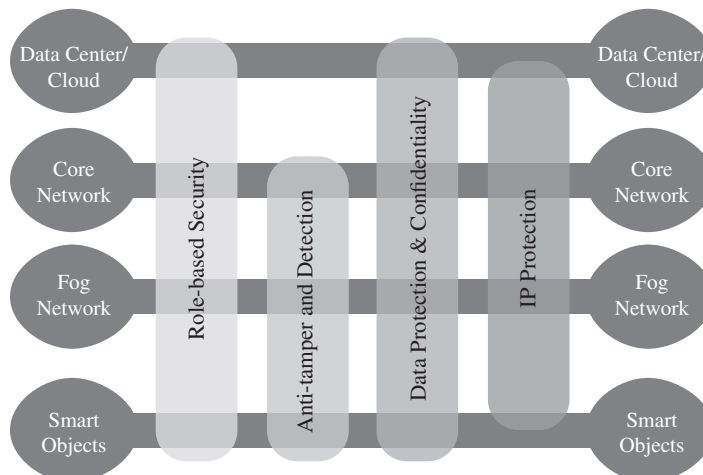
Figure 13.12 IoT Security Environment
