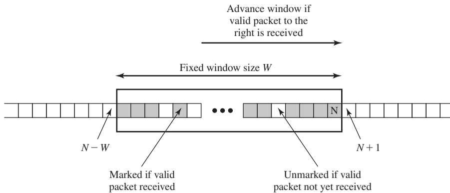
Figure 22.9 Antireplay Mechanism
