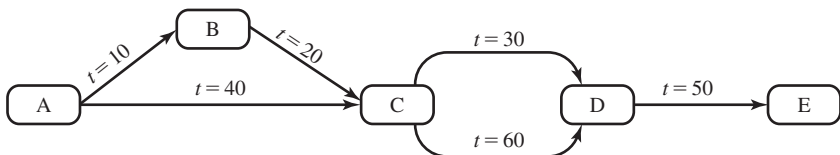
Figure 5.15 Cascaded Privileges
