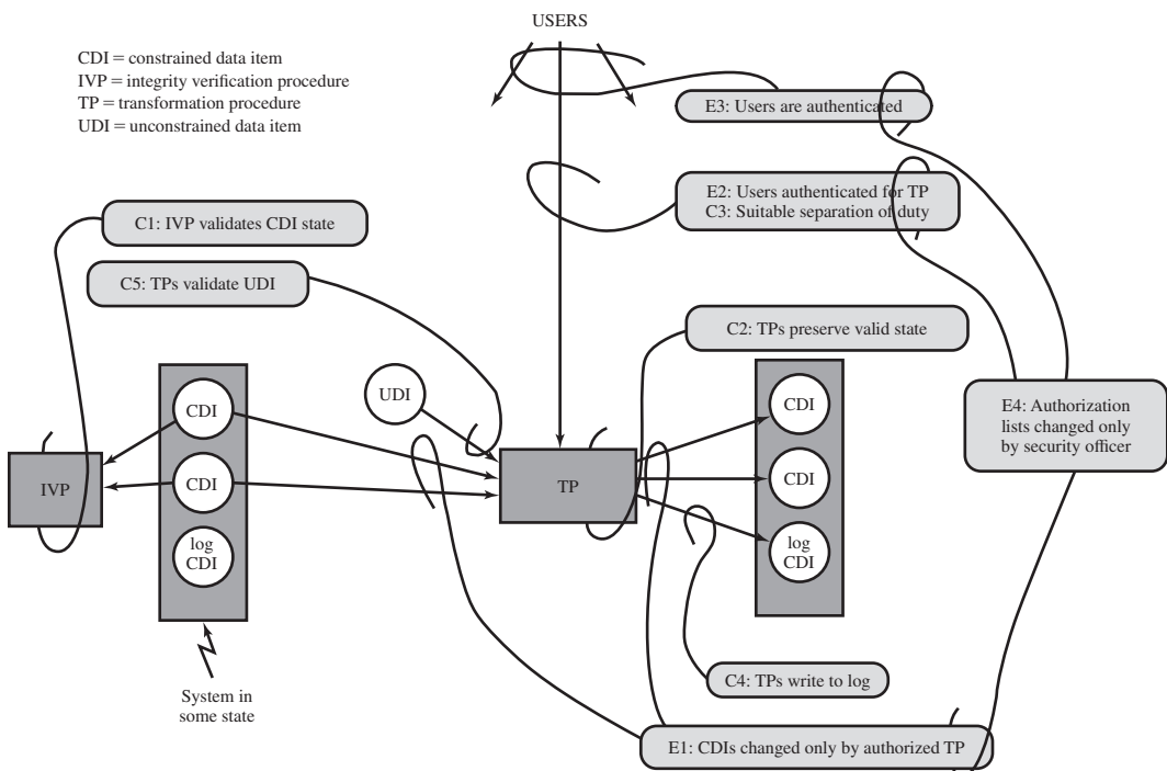
Figure 27.5 Summary of Clark-Wilson System Integrity Rules
