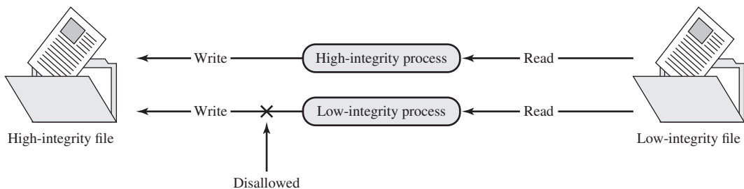
Figure 27.4 Contamination with Simple Integrity Controls
