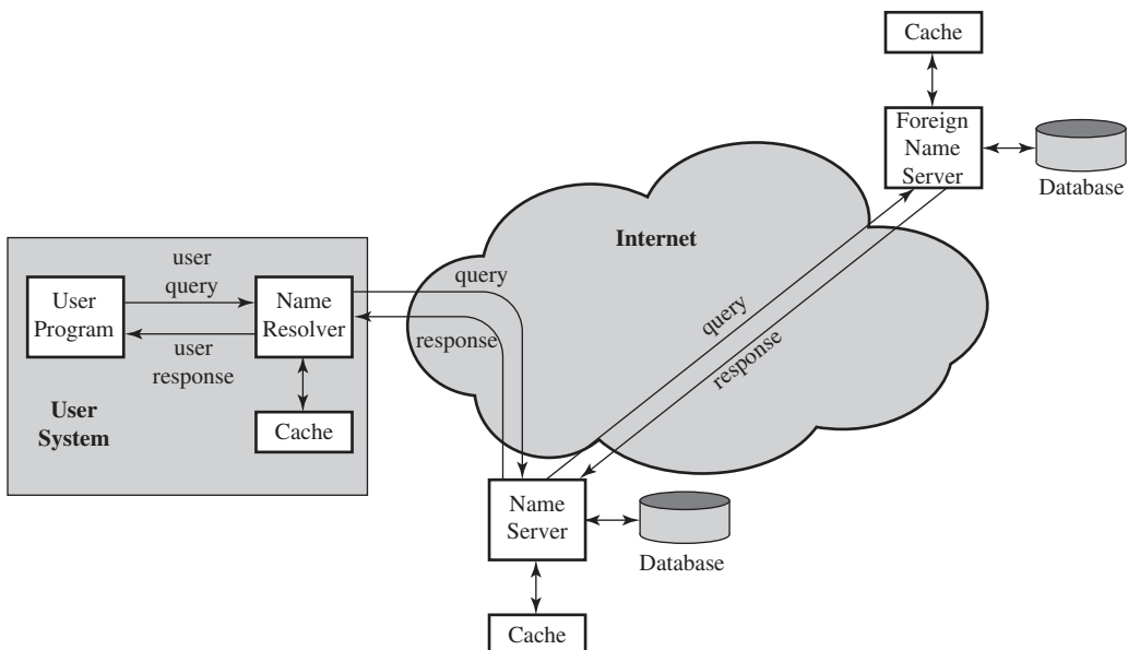
Figure H.3 DNS Name Resolution
