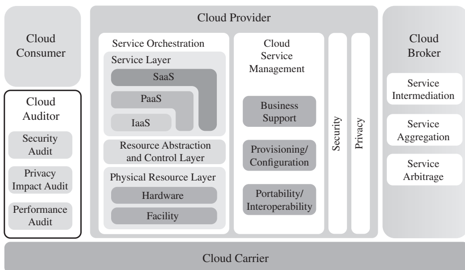
Figure 13.3 NIST Cloud Computing Reference Architecture
