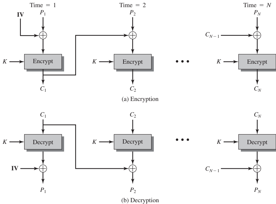
Figure 20.7 Cipher Block Chaining (CBC) Mode
