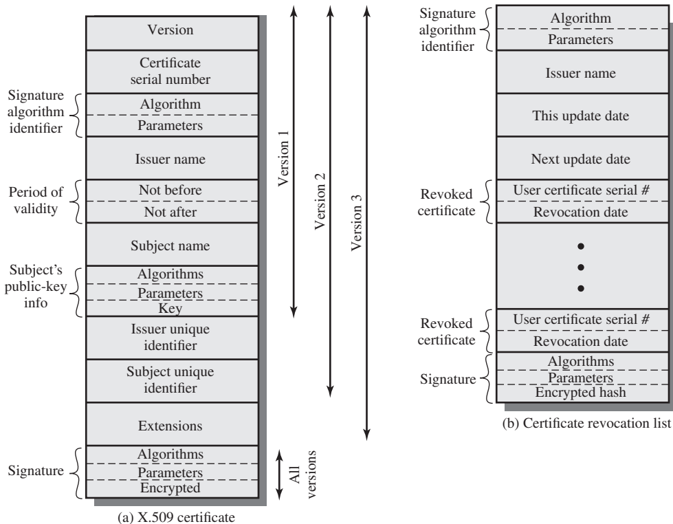
Figure 23.3 X.509 Formats
