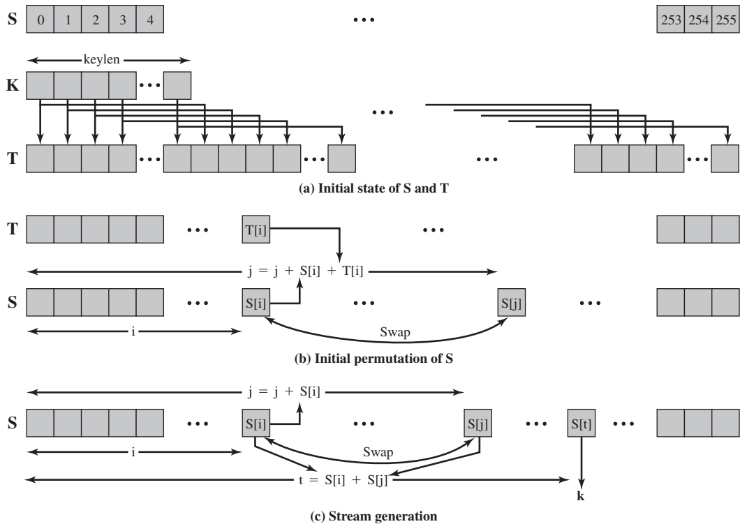
Figure 20.6 RC4
