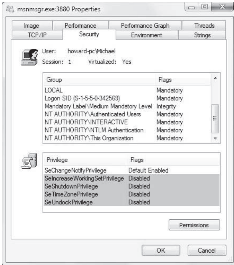
Figure 26.1 Screen Shot of User Account in Windows Vista
