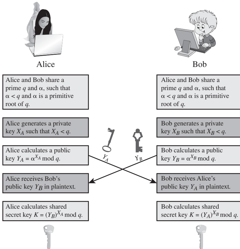
Figure 21.10 Diffie-Hellman Key Exchange
