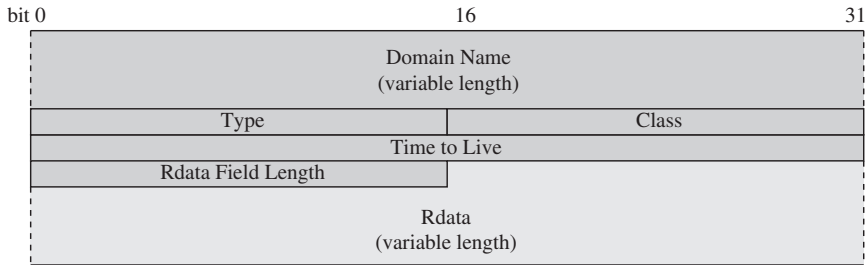
Figure H.2 DNS Resource Record Format
