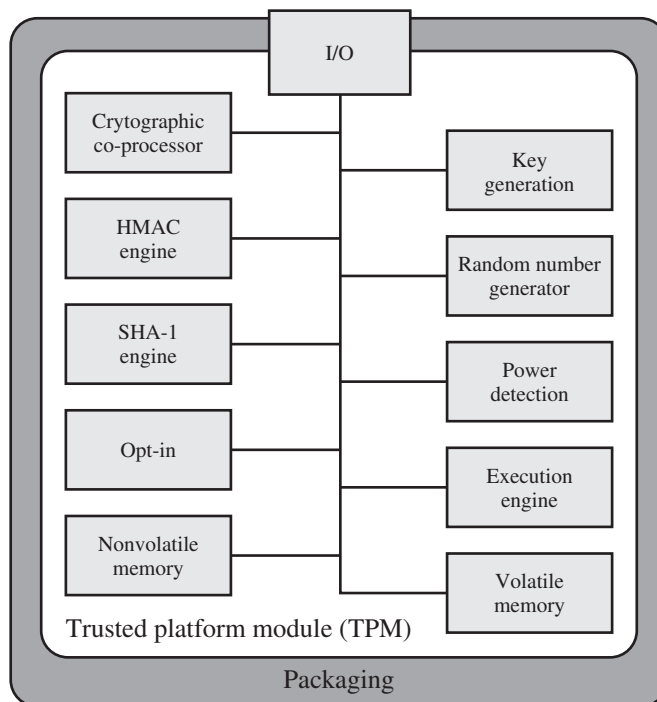
Figure 27.11 TPM Component Architecture
