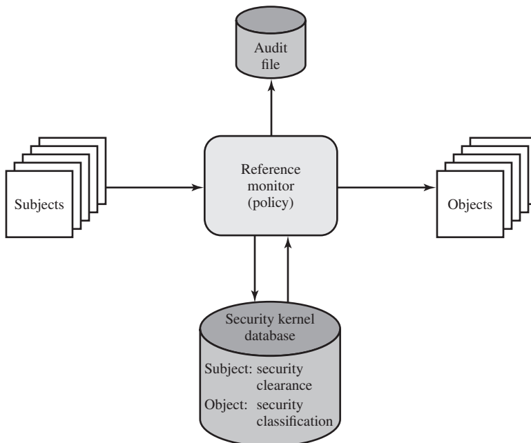
Figure 27.7 Reference Monitor Concept
