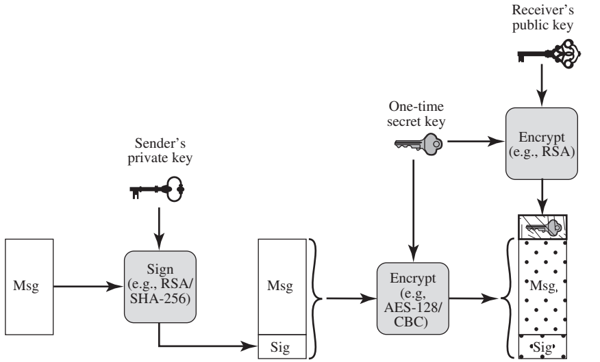
(a) Sender signs, and then encrypts message
