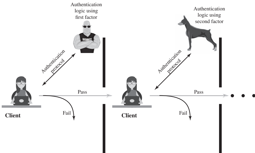
Figure 3.2 Multifactor Authentication
