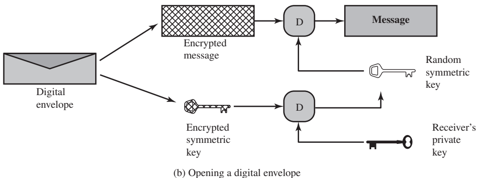
Figure 2.9 Digital Envelopes
