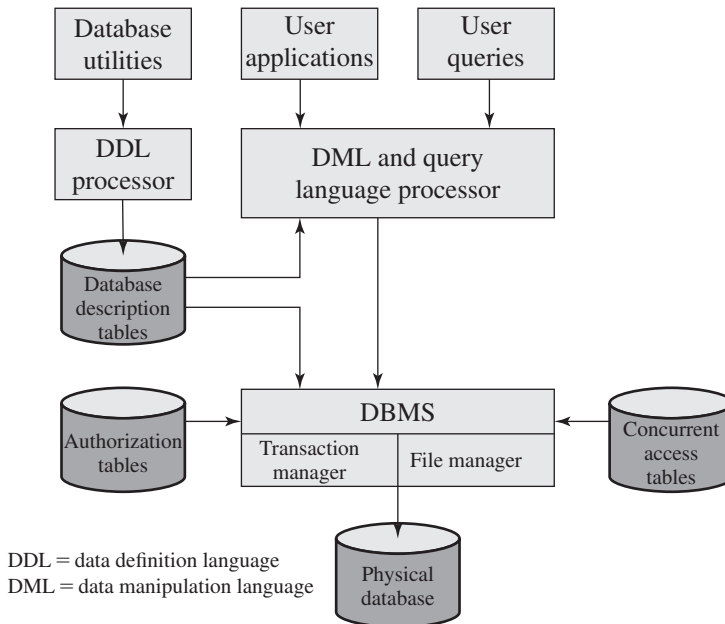
Figure 5.1 DBMS Architecture
