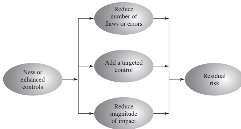
Figure 15.3 Residual Risk
