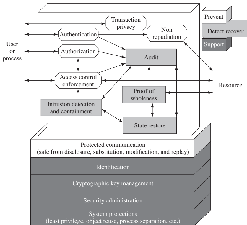
Figure 15.2 Technical Security Controls
