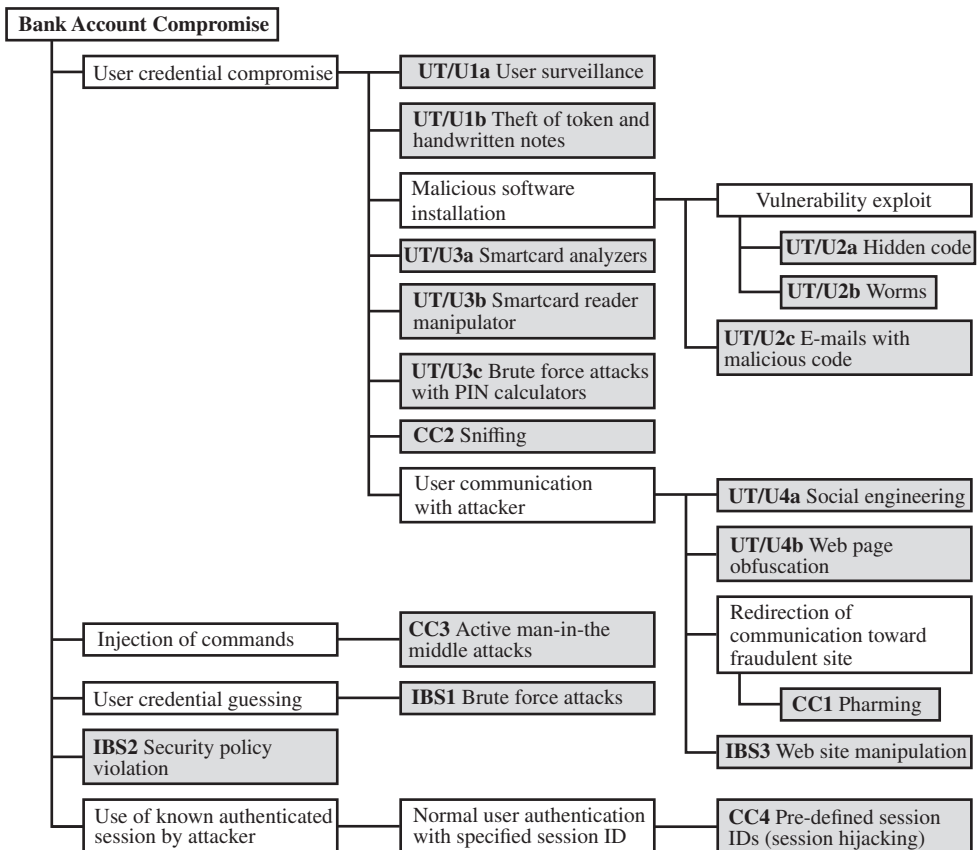
Figure 1.5 An Attack Tree for Internet Banking Authentication
