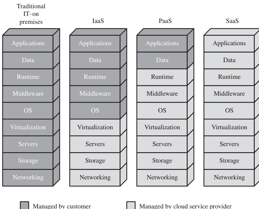
Figure 13.2 Separation of Responsibilities in Cloud Service Models
