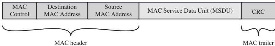
Figure 24.4 General IEEE 802 MPDU Format
