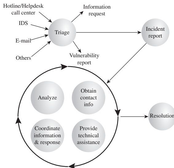
Figure 17.2 Incident Handling Life Cycle
