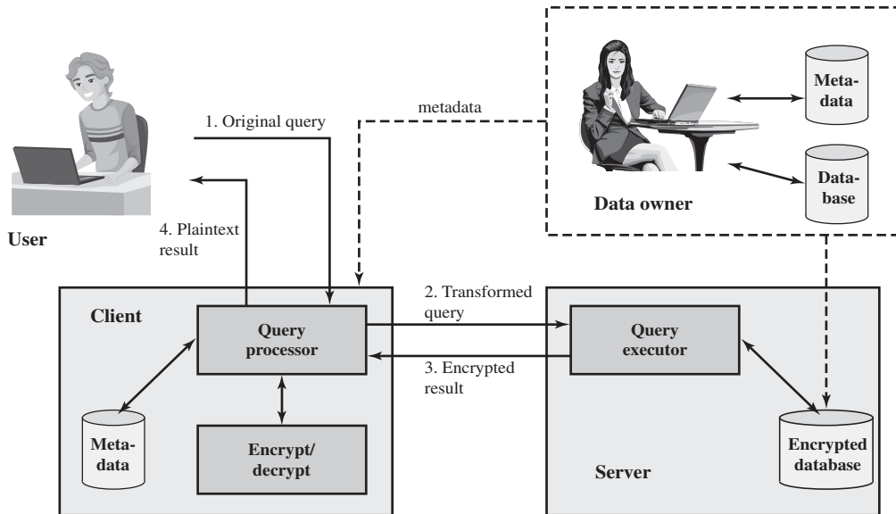
Figure 5.9 A Database Encryption Scheme
