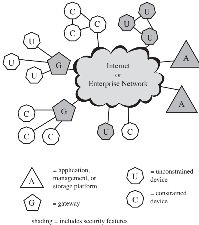
Figure 13.10 IoT Security: Elements of Interest
