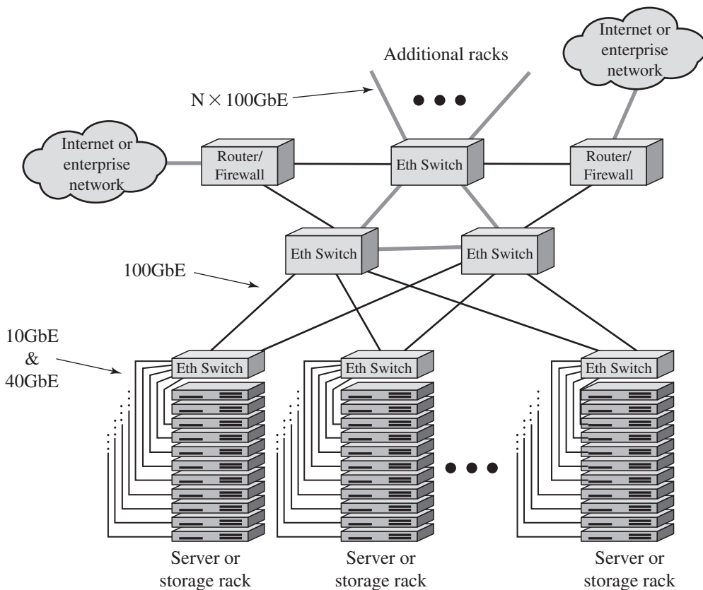
Figure 5.11 Key Data Center Elements
