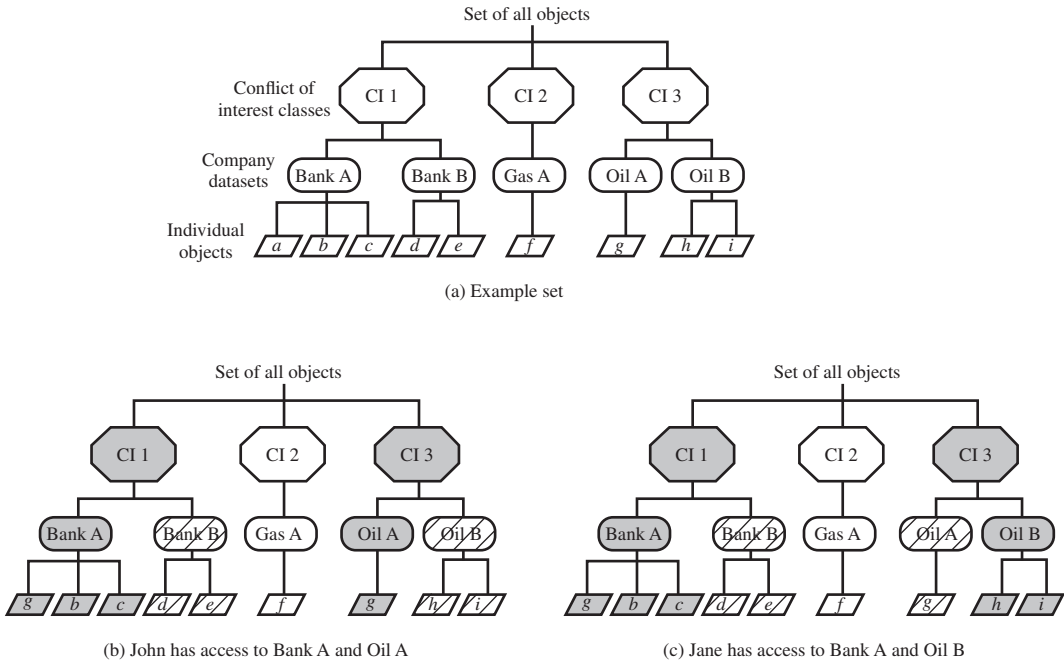
Figure 27.6 Potential Flow of Information between Two CIs
