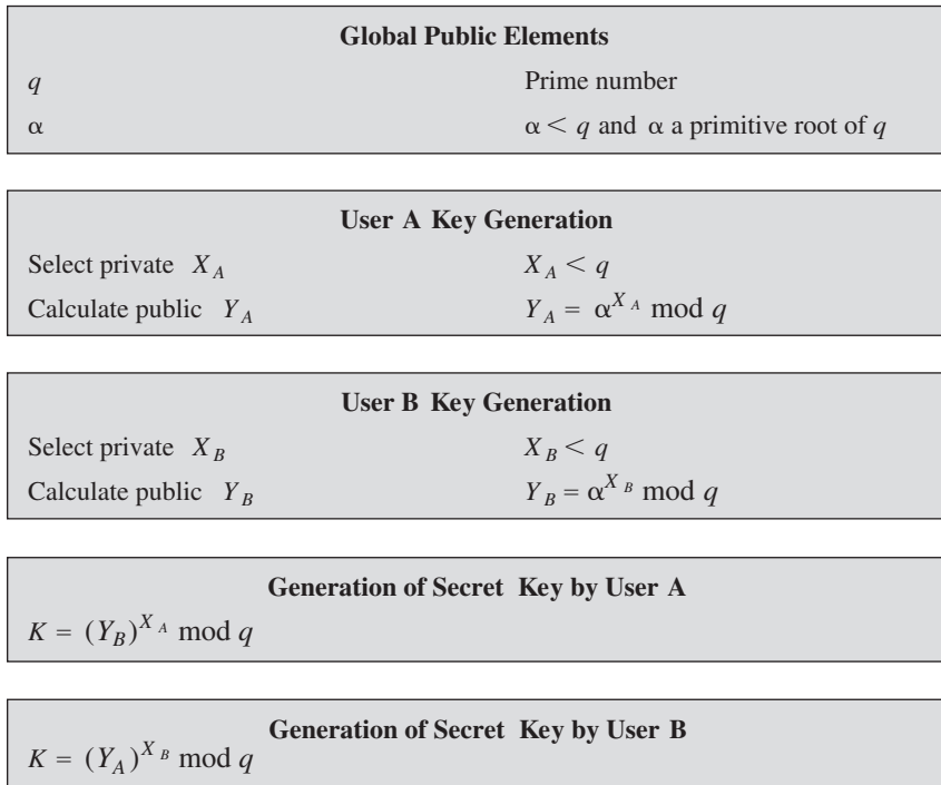
Figure 21.9 The Diffie-Hellman Key Exchange Algorithm
