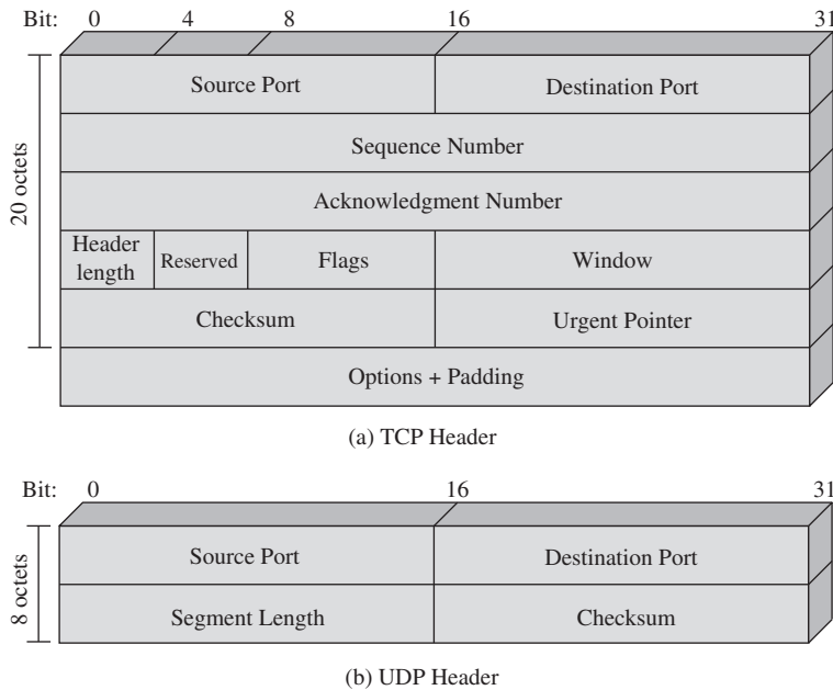
Figure F.1 TCP and UDP Headers
