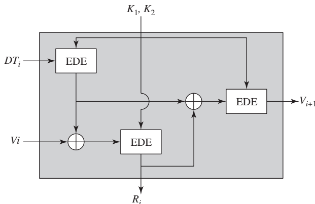
Figure D.2 ANSI X9.17 Pseudorandom Number Generator
