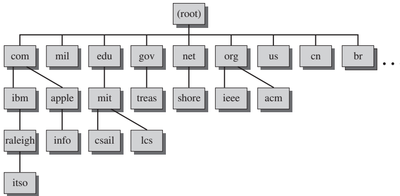
Figure H.1 Portion of Internet Domain Tree
