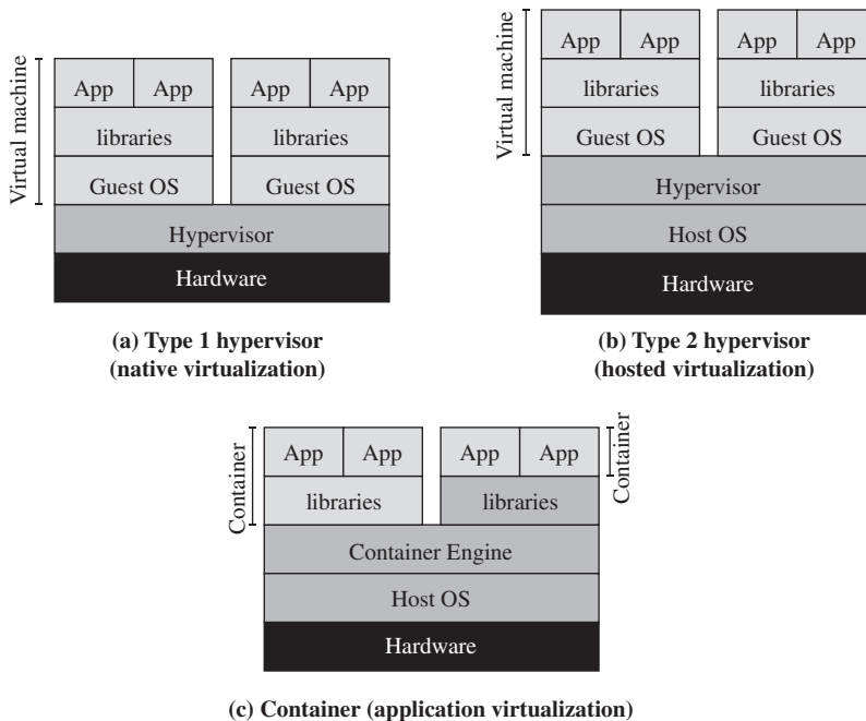
Figure 12.2 Comparison of Virtual Machines and Containers
