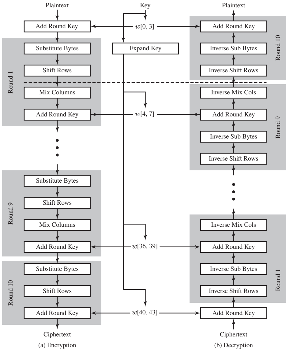
Figure 20.3 AES Encryption and Decryption
